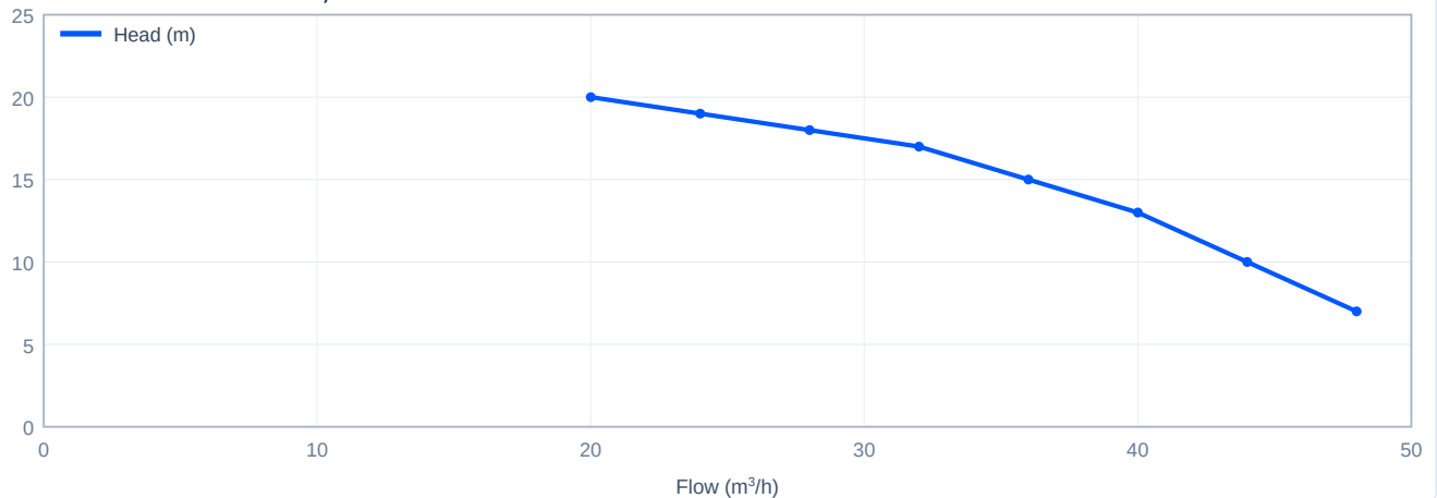
Head versus flow - CDL32-10-1, 60 Hz
