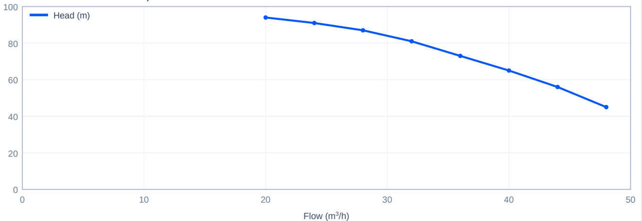
Head versus flow - CDL32-40-2, 60 Hz
