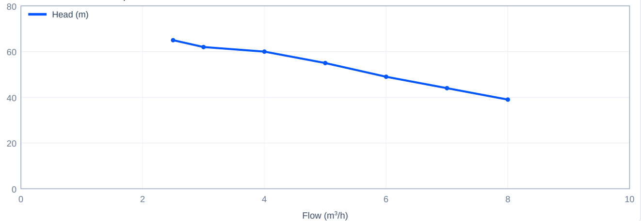
Head versus flow - CDL4-5, 60 Hz
