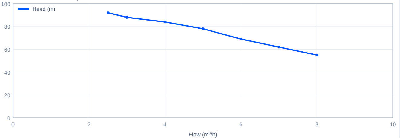
Head versus flow - CDL4-7, 60 Hz
