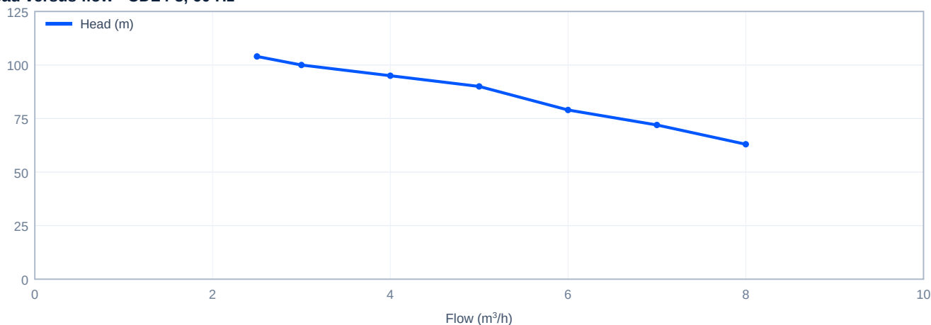
Head versus flow - CDL4-8, 60 Hz
