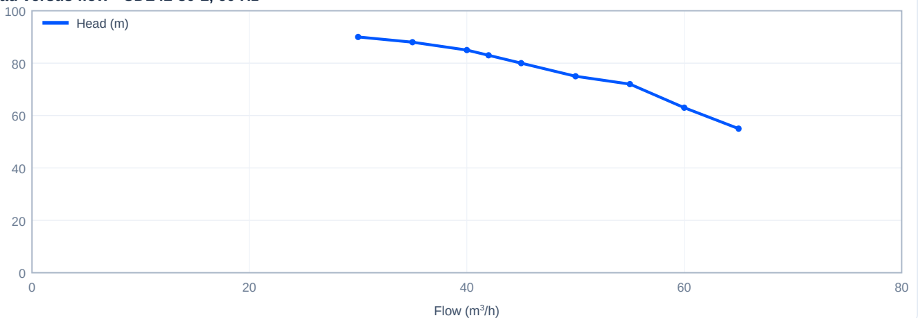
Head versus flow - CDL42-30-2, 60 Hz
