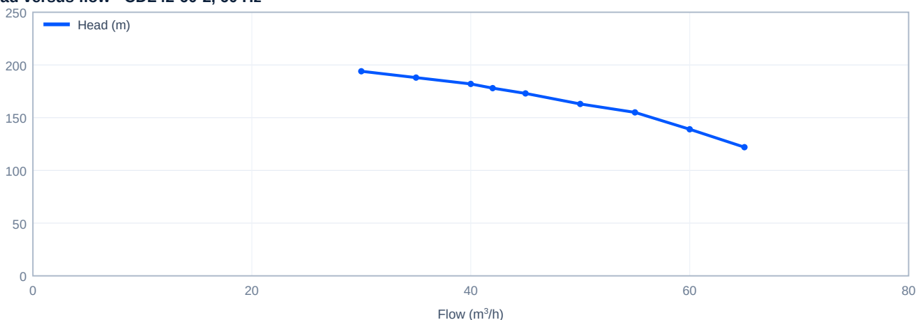
Head versus flow - CDL42-60-2, 60 Hz
