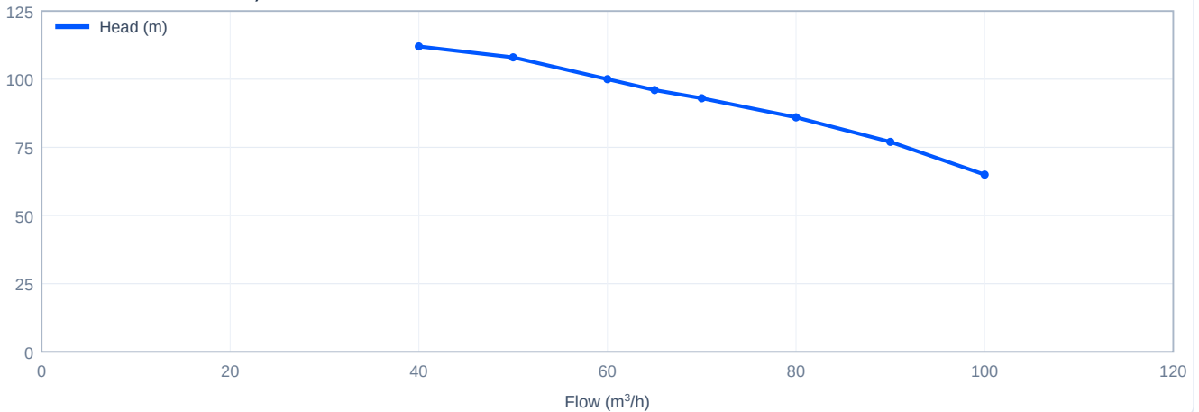
Head versus flow - CDL65-30, 60 Hz
