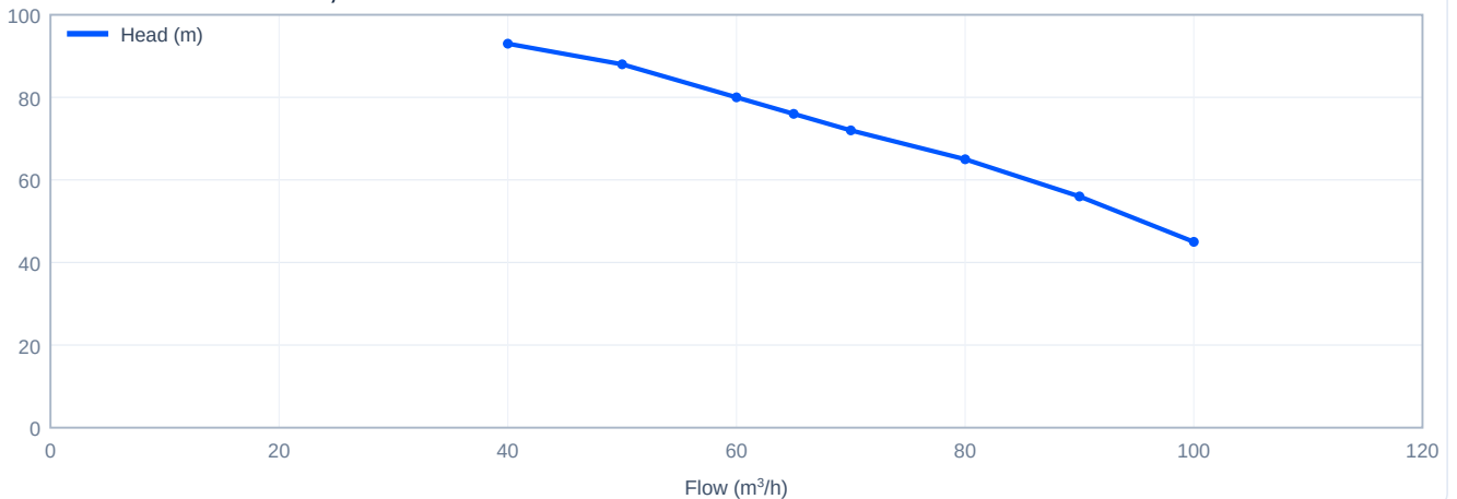
Head versus flow - CDL65-30-2, 60 Hz
