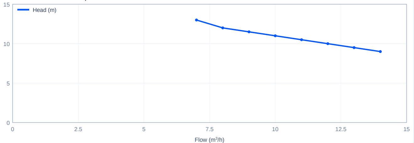
Head versus flow - CDL8-2/1, 60 Hz
