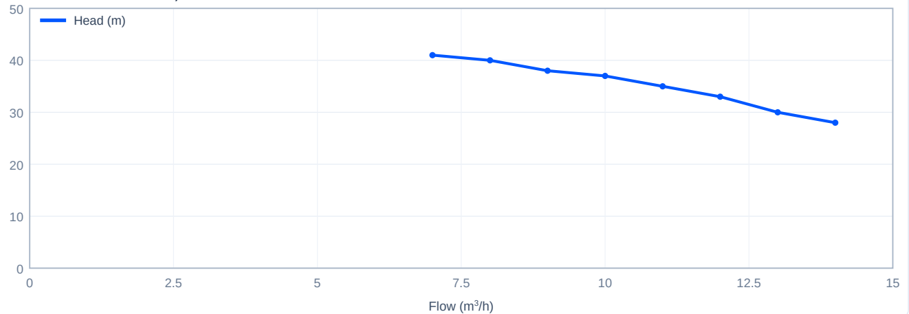
Head versus flow - CDL8-3, 60 Hz
