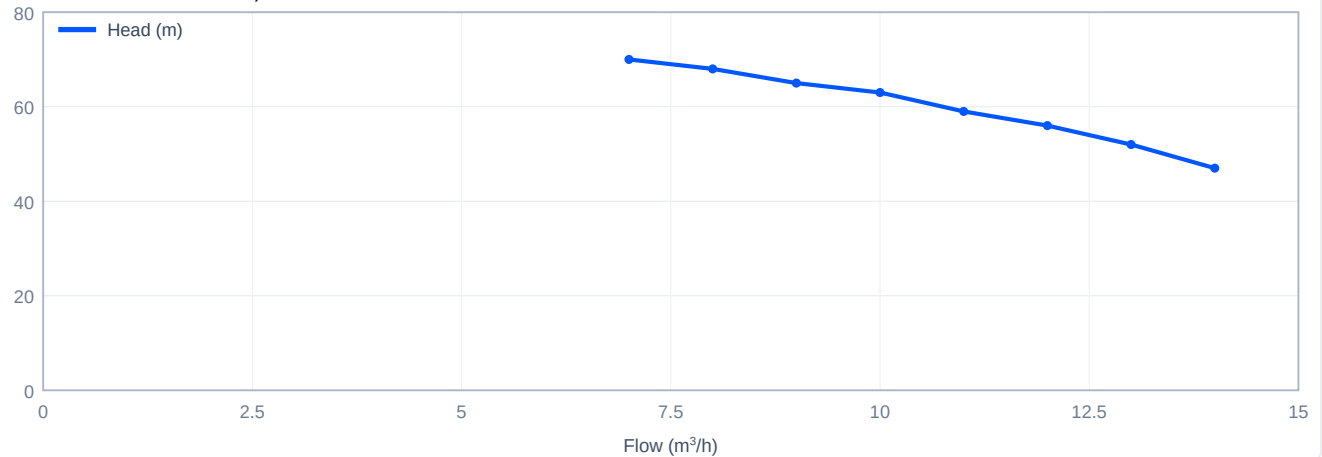
Head versus flow - CDL8-5, 60 Hz
