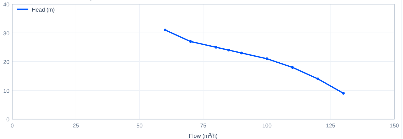
Head versus flow - CDL85-10-1, 60 Hz
