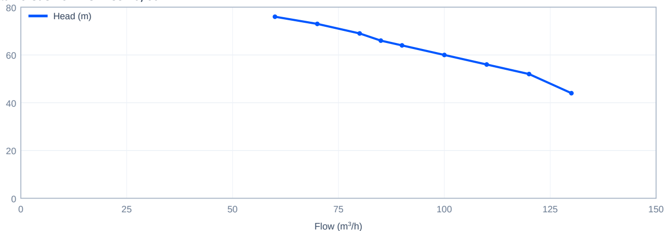
Head versus flow - CDL85-20, 60 Hz
