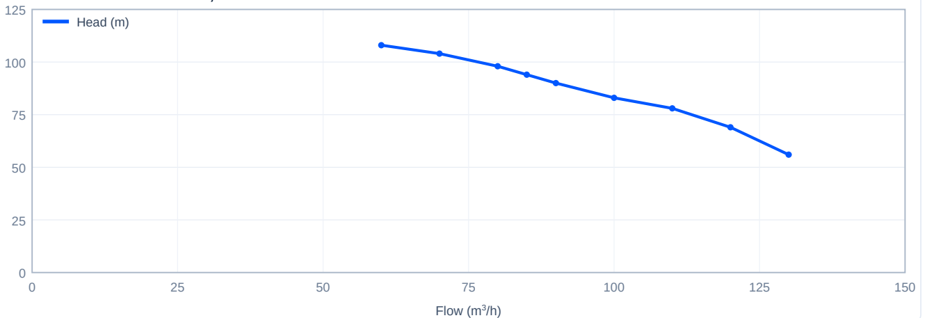
Head versus flow - CDL85-30-1, 60 Hz
