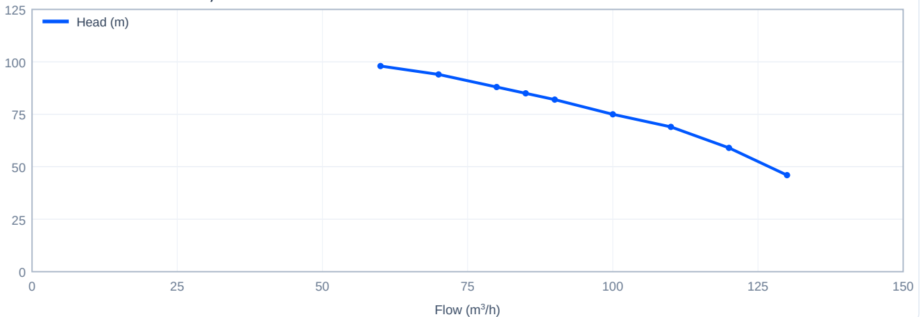
Head versus flow - CDL85-30-2, 60 Hz
