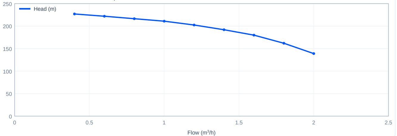
Head versus flow - CDLF1-3+CDH1-36, 50 Hz
