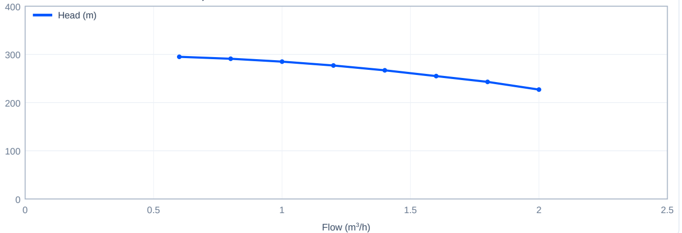
Head versus flow - CDLF1-10+CDH1-25, 60 Hz
