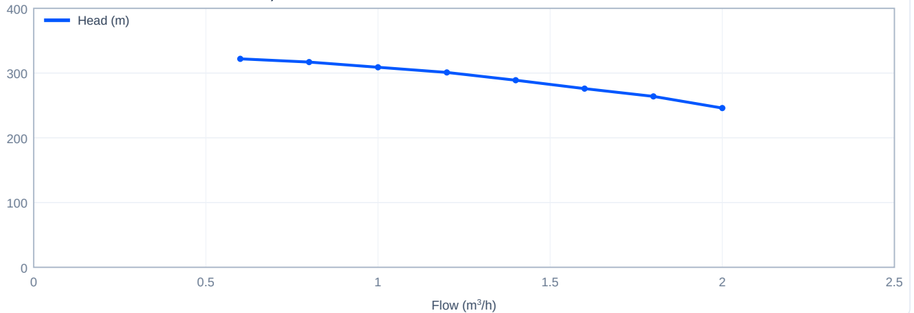
Head versus flow - CDLF1-13+CDH1-25, 60 Hz
