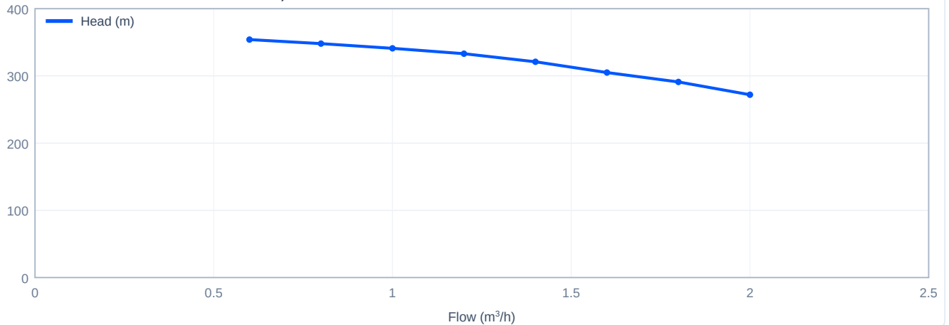
Head versus flow - CDLF1-17+CDH1-25, 60 Hz
