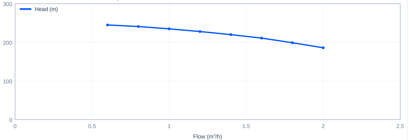
Head versus flow - CDLF1-4+CDH1-25, 60 Hz
