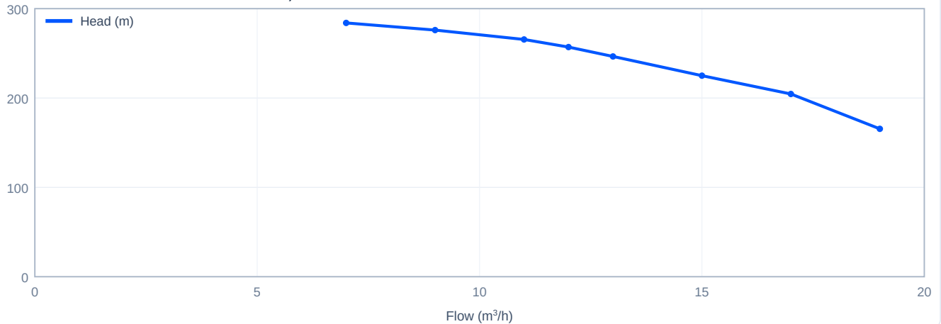
Head versus flow - CDLF12-2+CDH12-14, 60 Hz
