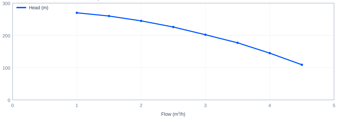
Head versus flow - CDLF2-3+CDH2-18, 60 Hz
