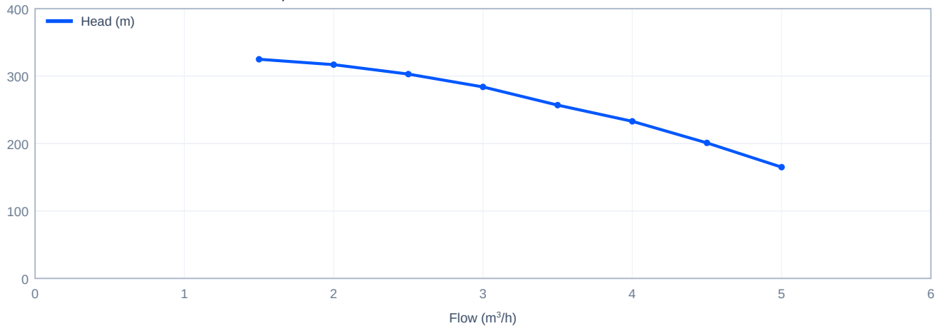
Head versus flow - CDLF3-13+CDH3-25, 60 Hz
