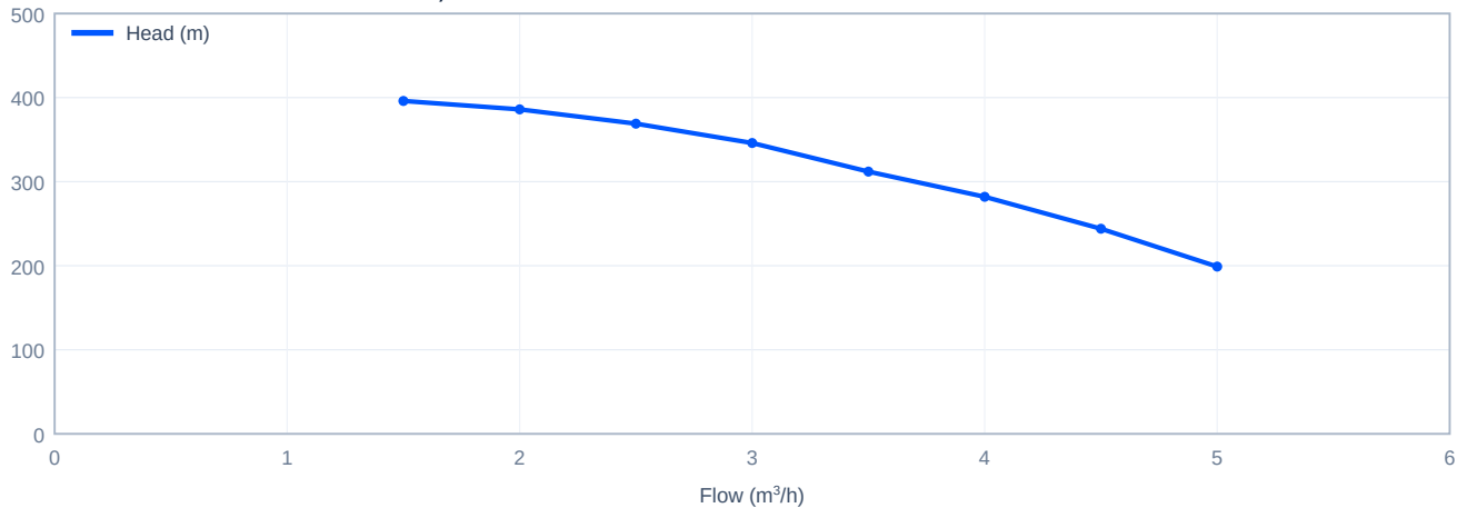
Head versus flow - CDLF3-21+CDH3-25, 60 Hz
