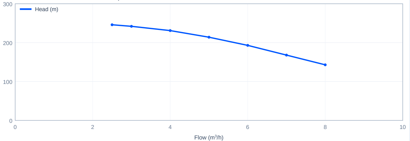
Head versus flow - CDLF4-3+CDH4-16, 60 Hz
