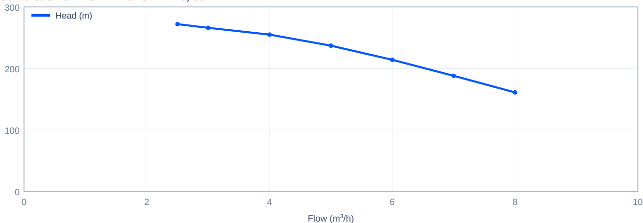
Head versus flow - CDLF4-5+CDH4-16, 60 Hz
