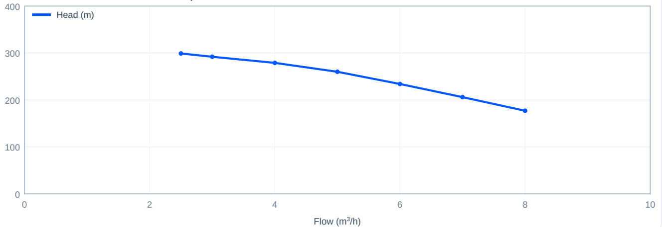
Head versus flow - CDLF4-7+CDH4-16, 60 Hz
