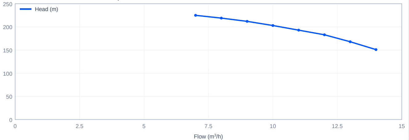
Head versus flow - CDLF8-2+CDH8-14, 60 Hz
