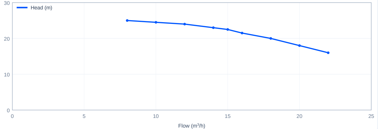
Head versus flow - CDLK15-20/2, 50 Hz
