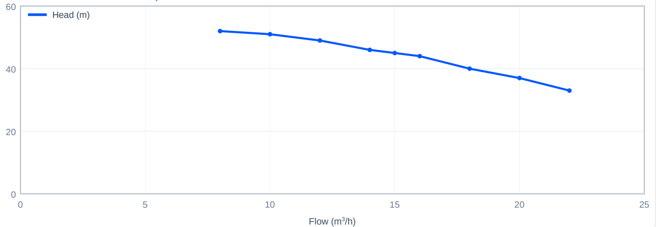
Head versus flow - CDLK15-40/4, 50 Hz
