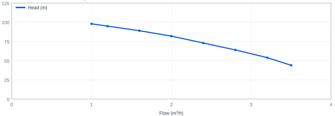
Head versus flow - CDLK2-110/11, 50 Hz
