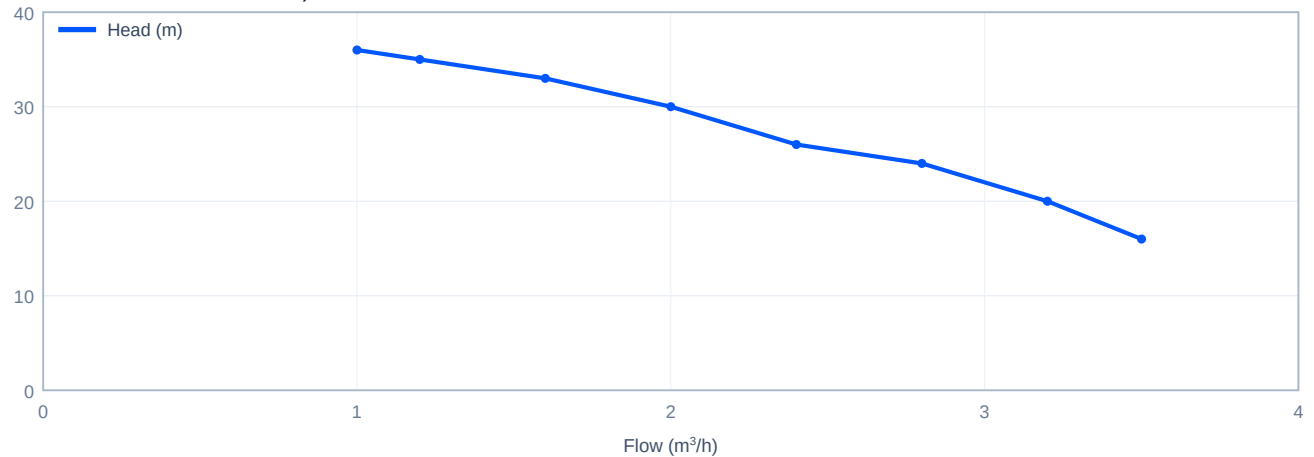
Head versus flow - CDLK2-40/4, 50 Hz
