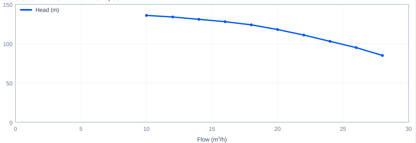
Head versus flow - CDLK20-100/10, 50 Hz
