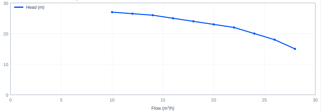
Head versus flow - CDLK20-20/2, 50 Hz
