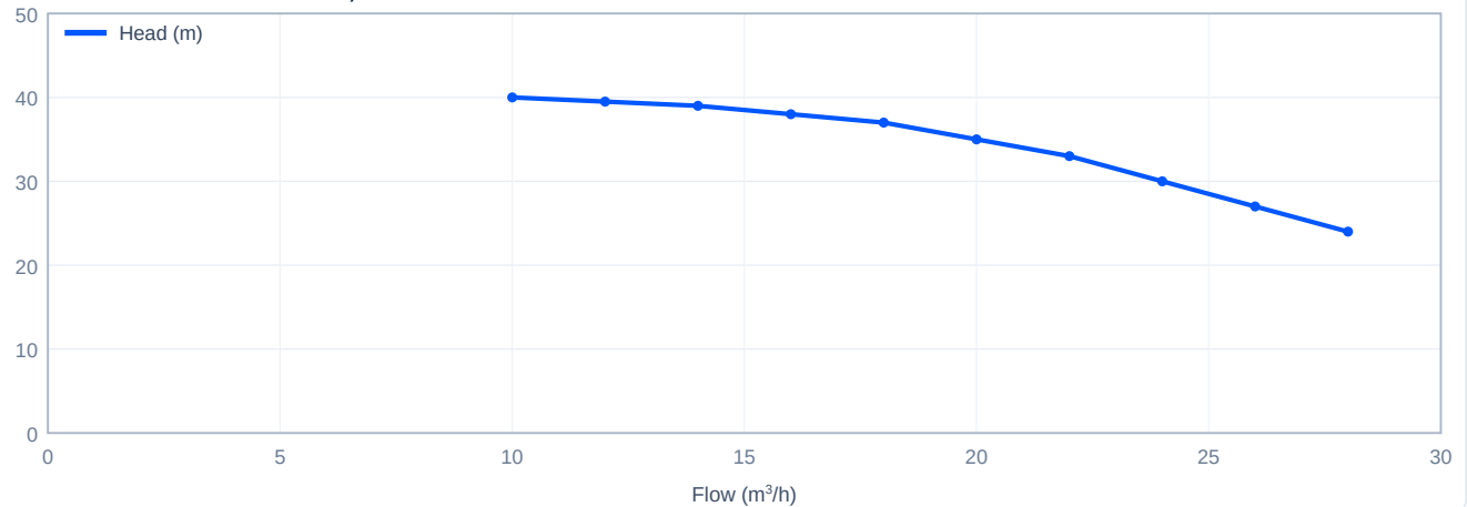
Head versus flow - CDLK20-30/3, 50 Hz
