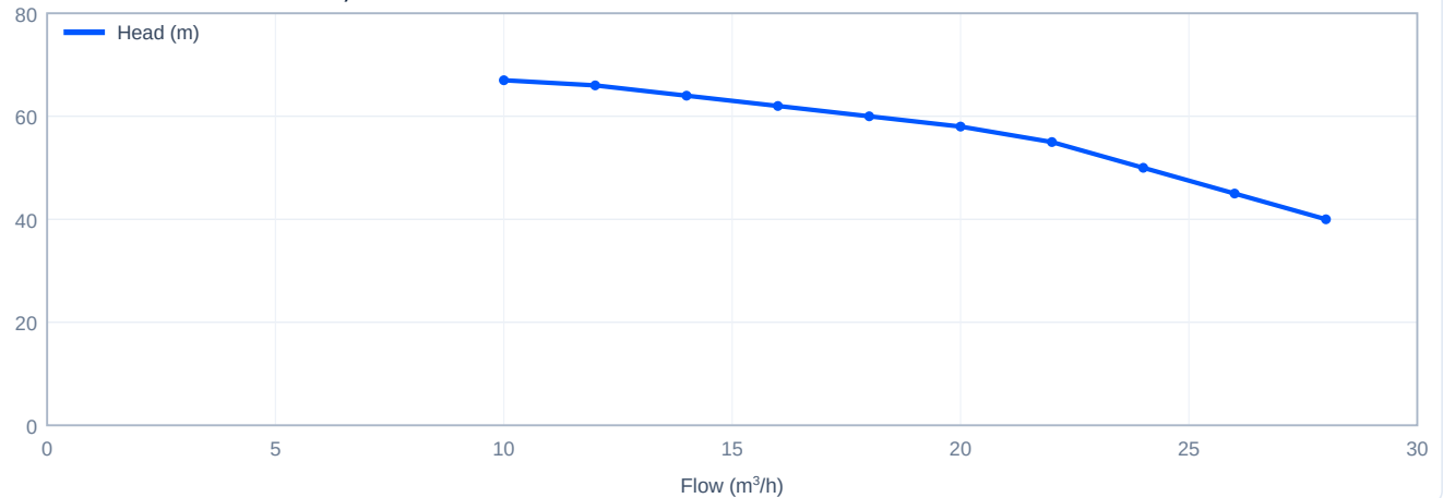
Head versus flow - CDLK20-50/5, 50 Hz
