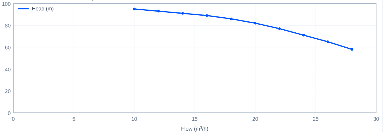
Head versus flow - CDLK20-70/7, 50 Hz
