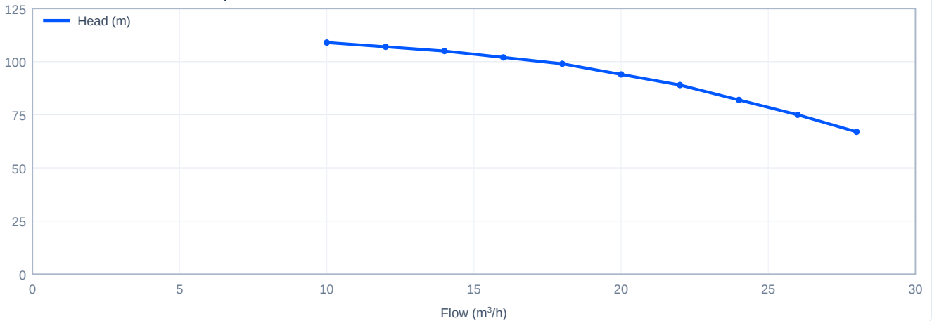
Head versus flow - CDLK20-80/8, 50 Hz
