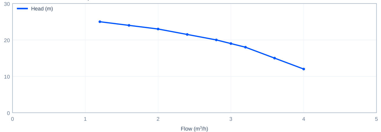
Head versus flow - CDLK3-40/4, 50 Hz
