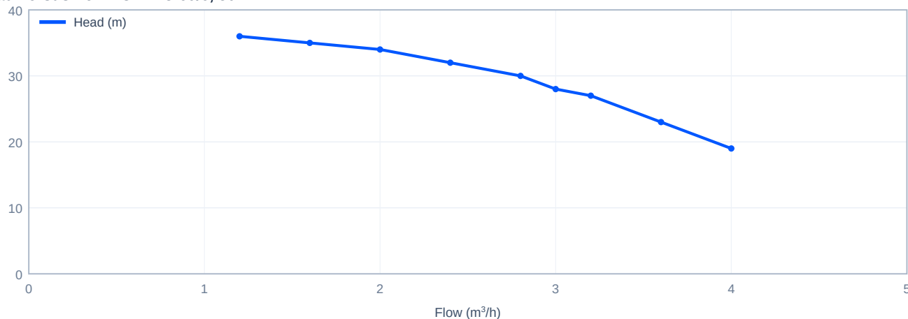
Head versus flow - CDLK3-60/6, 50 Hz
