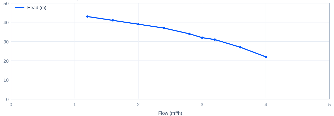
Head versus flow - CDLK3-70/7, 50 Hz
