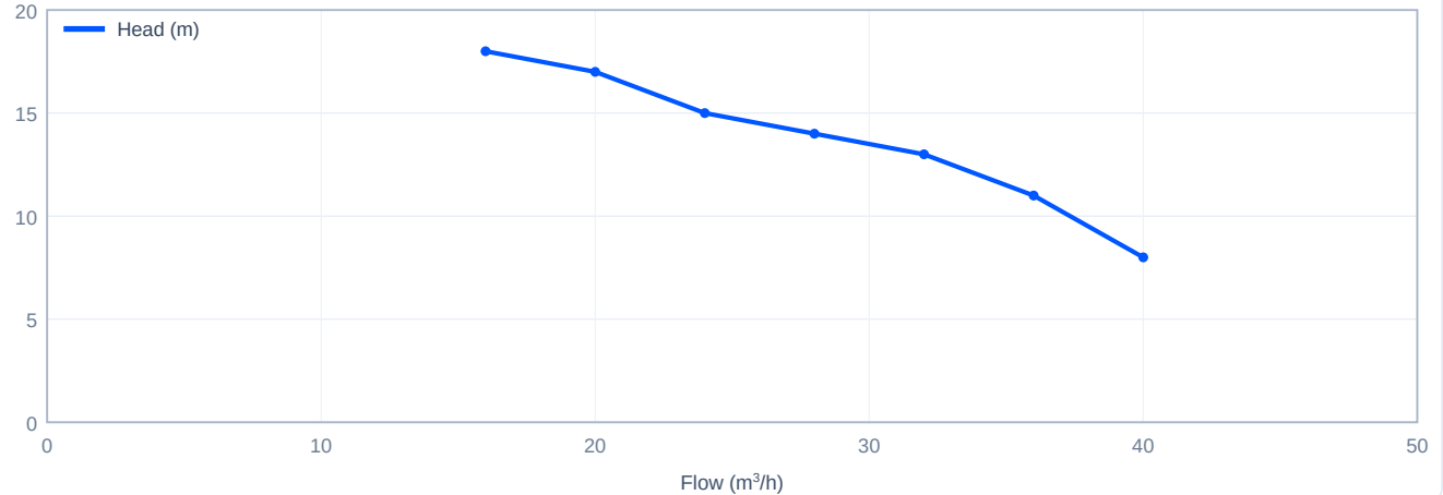
Head versus flow - CDLK32-10/1, 50 Hz
