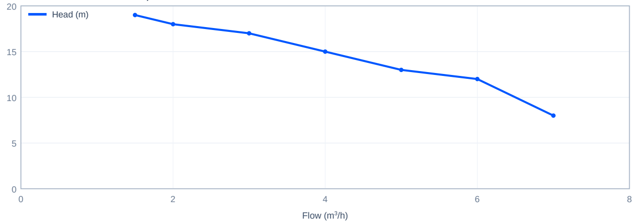
Head versus flow - CDLK4-20/2, 50 Hz
