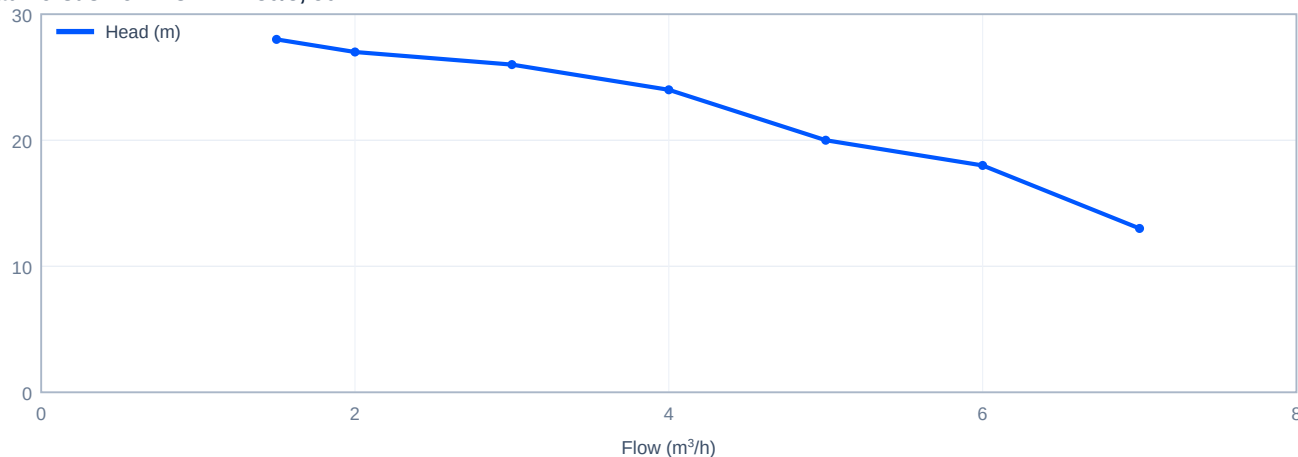
Head versus flow - CDLK4-30/3, 50 Hz
