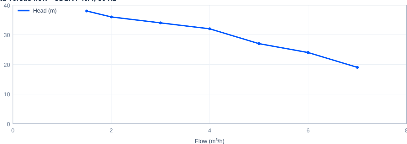
Head versus flow - CDLK4-40/4, 50 Hz
