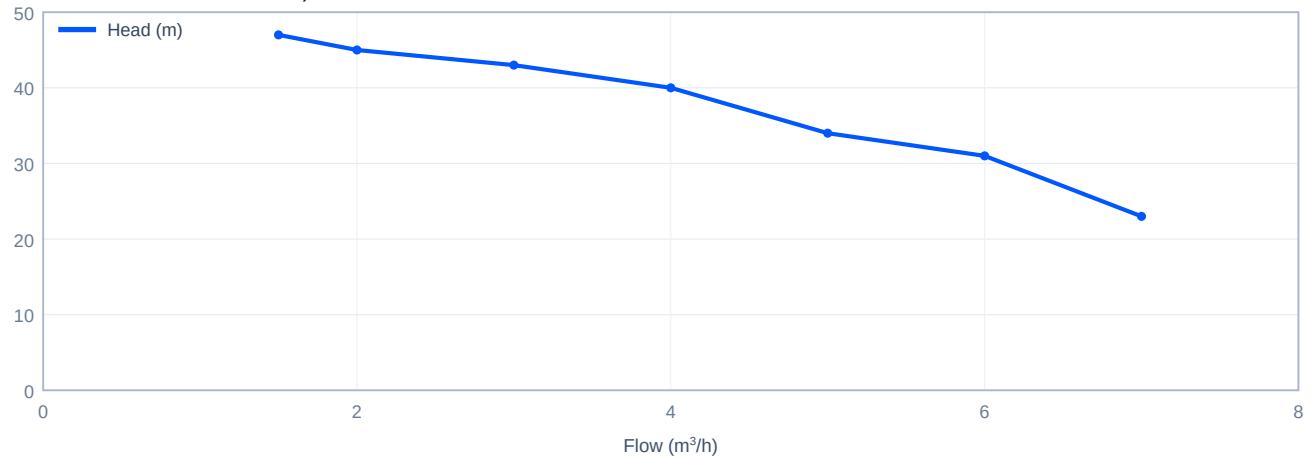
Head versus flow - CDLK4-50/5, 50 Hz
