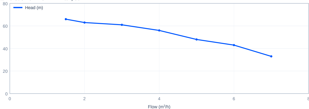
Head versus flow - CDLK4-70/7, 50 Hz
