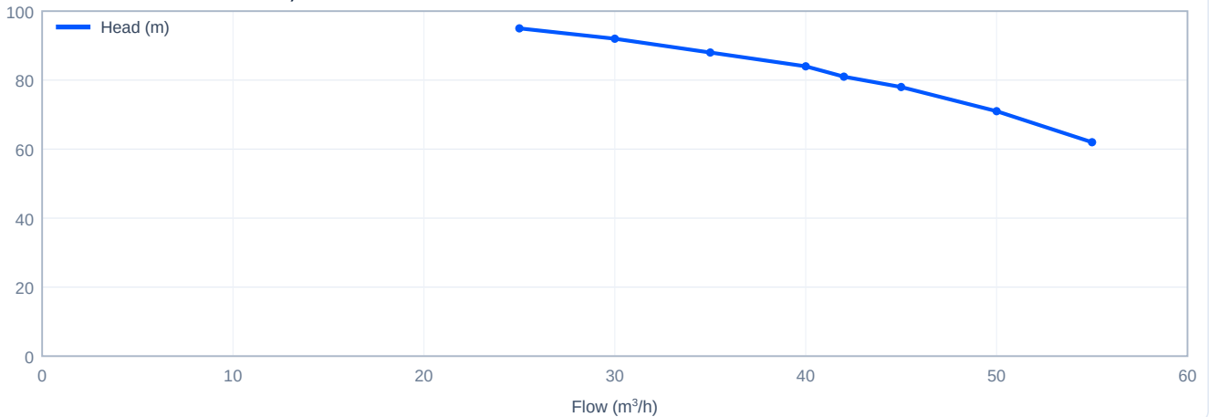
Head versus flow - CDLK42-40/4, 50 Hz
