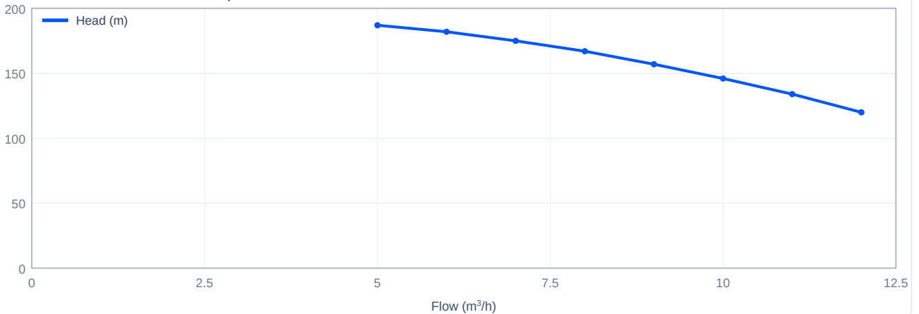
Head versus flow - CDLK8-180/18, 50 Hz
